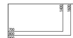
Rectangular high table
