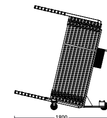
Stacking trolley 6398-000 (example with table length 1600)
